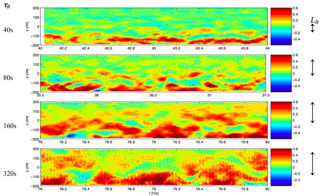
Figure 2 Azimuthal mean zonal (azimuthal) velocity (in \text{cm s}^{-1} ) as a function of time within the field imaged by both cameras of the experiment, obtained at mid-depth of the tank. Four different rotation rates are shown, leading to values of \beta L^2/U of 25 – 500. Jets scale roughly with the Rhines scale L_R , indicated by the arrows on the right.
