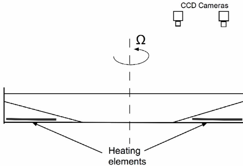
Figure 1: Schematic cross-section of tank, showing sloping bottom boundary and location of heating elements. The flow was viewed from above by two CCD cameras located along a radius.
