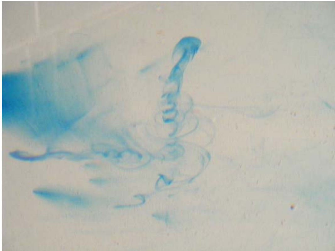
Figure 3: Photograph of a convective thermal plume rising from the bottom of the tank, visualized by blue dye. The plume is the core of a cyclonically circulating vortex of diameter ~10-20 cm and around 30 cm high.
