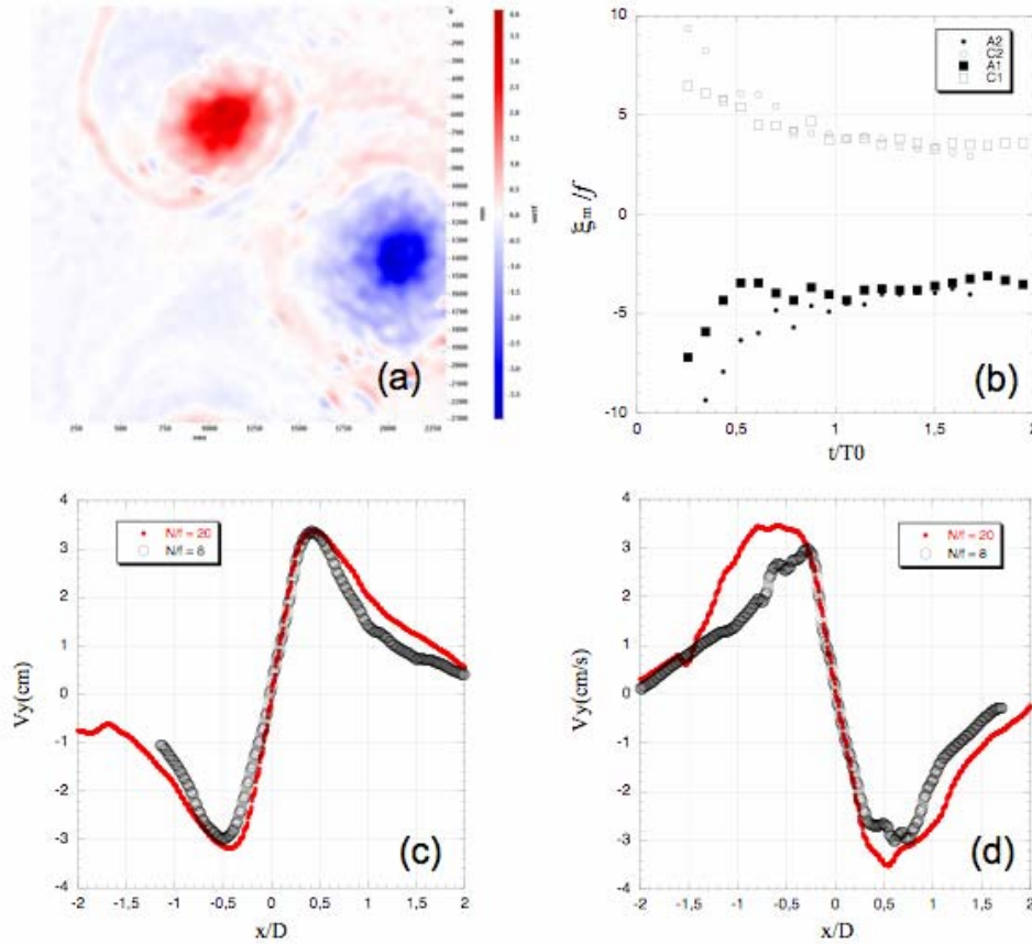
Figure 1 Relative vorticity of cyclonic (red) and anticyclonic (blue) eddies (a); core vorticity evolution (b); cyclonic (c) and anticyclonic (d) velocity profiles corresponding to the parameters: Re \sim 1700 , Ro \sim 2 , d=0.25 and S=8 and S=20 .
