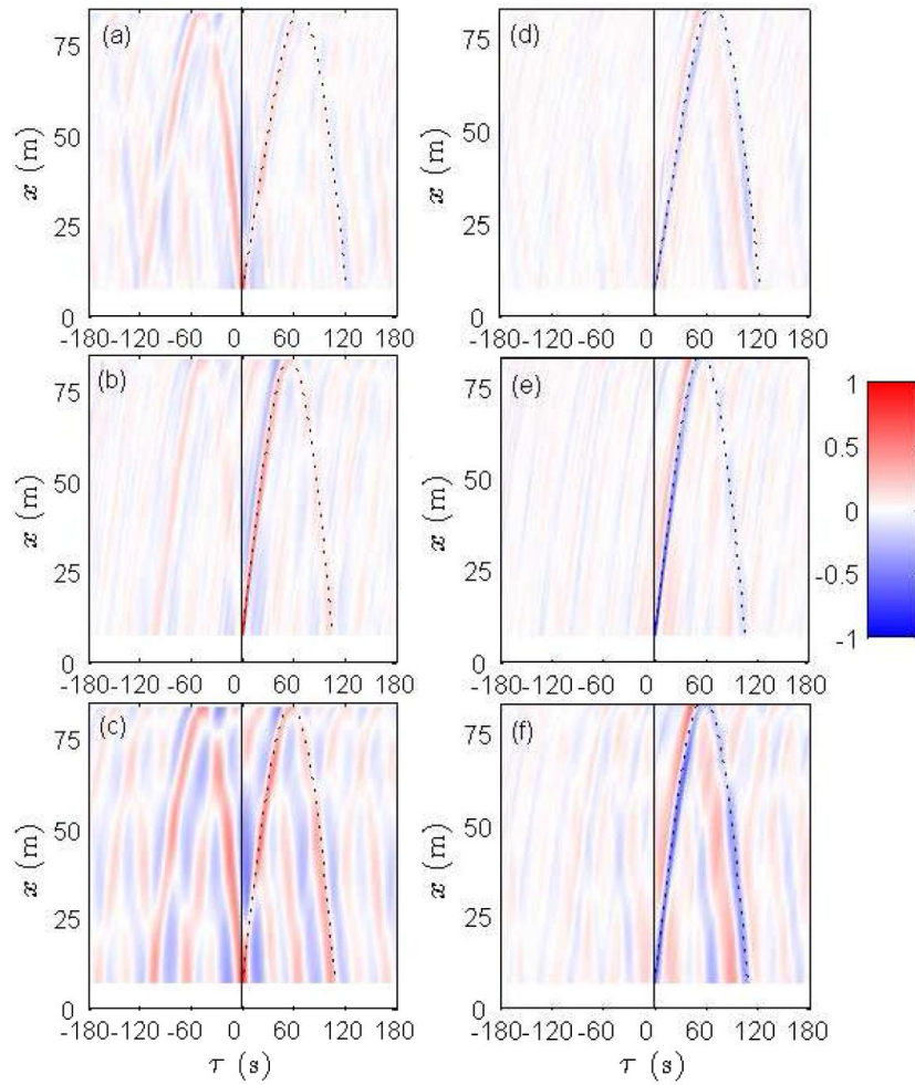
Figure 5. Correlation functions of the infragravity wave at all positions to a fixed reference position x = 5.6 m (a) A1, (b) A2, and (c) A3, and cross-correlation functions between the squared short wave envelope at a fixed reference position x = 5.6 m and the infragravity wave as observed at all locations (d) A1, (e) A2, and (f) A3. The solid line represents time lag ( \tau ) is zero. Dashed lines indicate time lag values (calculated as described in Ruju et al., 2012) for shoreward propagating waves at group speed c_g , and in the offshore direction at \sqrt{gh} . Red colors indicate positive correlations, blue colors indicate negative correlations.
