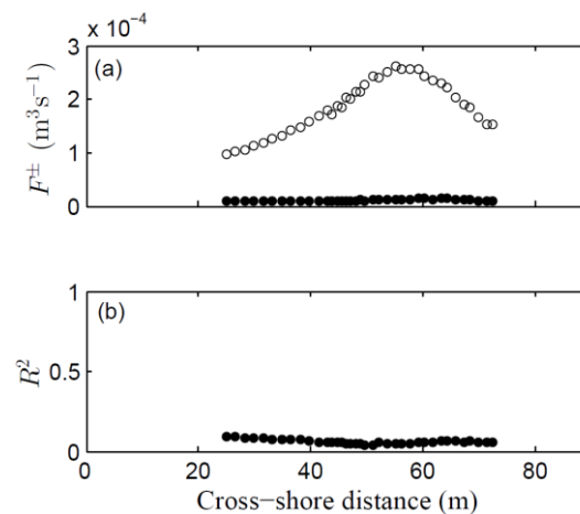
Figure 7. (a) Bulk incoming (circles) and outgoing (black dots) infragravity energy fluxes ( F^{\pm} ) for A2 and (b) bulk reflection coefficients ( R^2 ) for the infragravity wave band for A2.
