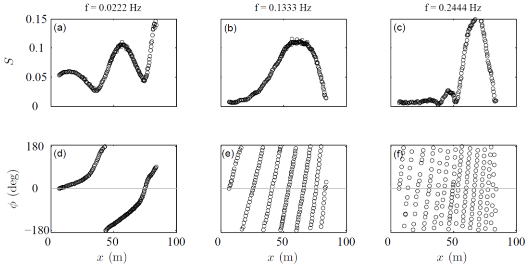
Figure 6. (a-c) Non-dimensional amplitude S and (d-f) phase \phi for A2 were computed from the dominant Empirical Orthogonal Function of the cross-spectral matrix for each period. The cross-spectra were computed from 50% overlapping, Hamming-windowed series.
