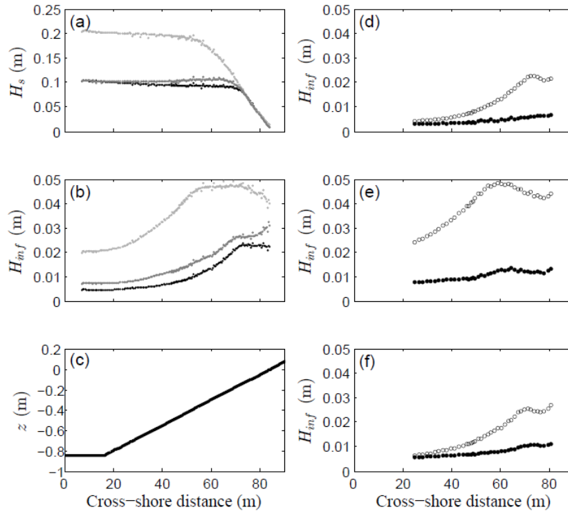
Figure 1. Significant wave height versus cross-shore distance x for (a) short waves H_s and (b) infragravity waves H_{inf} for A1 (black dots), A2 (light-grey dots) and A3 (dark-grey dots). (c) Bed profile. Furthermore, the significant incoming (circles) and outgoing (black dots) infragravity-wave heights calculated from separated signals (following Guza et al., 1984) are shown for (d) A1, (e) A2 and (f) A3.
