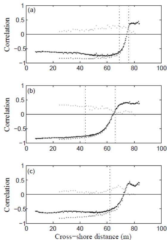
Figure 4. Correlations r at \tau = 0 between the short-wave envelope and the separated and total infragravity wave signal (a) A1, (b) A2 and (c) A3 with total infragravity wave signal (black dots), incoming infragravity wave signal (dark-grey dots) and outgoing infragravity wave signal (light-grey dots). Dashed lines are the visually determined location where (left) the largest short waves started to break, and (right) where all waves broke. The single line in (c) shows the initiation of short wave breaking, due to the narrow-banded spectrum the waves break close together.
