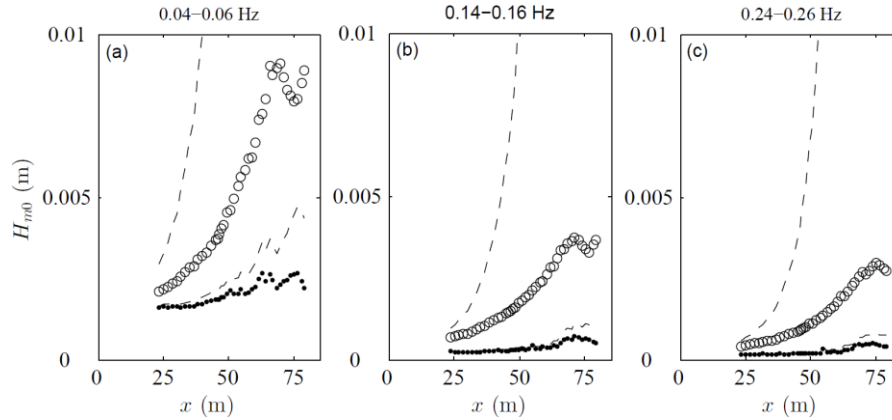
Figure 3. Incoming (circles) and outgoing (black dots) significant infragravity wave height for three frequency bands of case A3, (a) 0.04-0.06 Hz, (b) 0.14-0.16 Hz and (c) 0.24-0.26 Hz. Green's law (lower dashed line) and the shallow-water asymptote of the Longuet-Higgins and Stewart (1962) equilibrium solution (upper dashed line).
