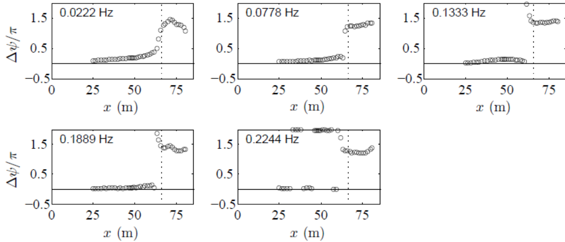
Figure 2. Additional phase lag ( \Delta\phi ) of the infragravity wave behind the short wave envelope for 5 different frequencies for condition A2. The dashed line in the figures is the location where all short waves were observed to break.
