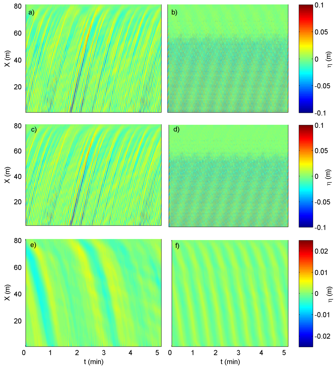
Figure 2. Surface elevation \eta spatiotemporal evolution along the cross-shore direction X (m). a) Total A2, b) total B2, c) incoming A2, d) incoming B2, e) outgoing A2 and f) outgoing B2 waves fields.
