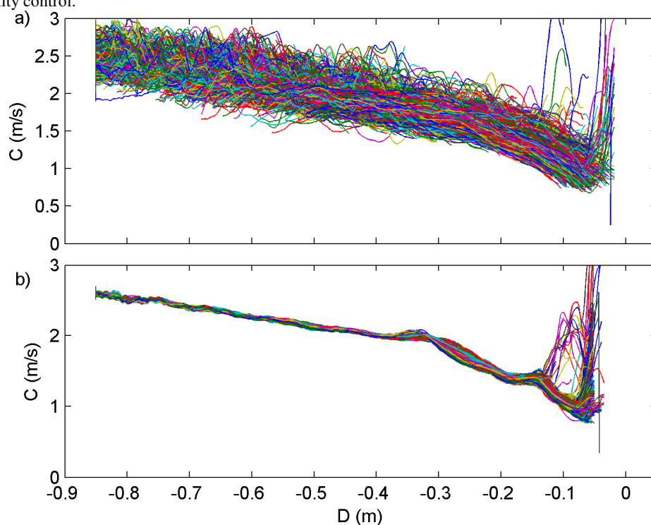
Figure 6. Individual wave ( \sim 1000 ) celerities C estimated from the trajectory tracking method as function of depth D (m) for the a) A2 and b) B2 series.
