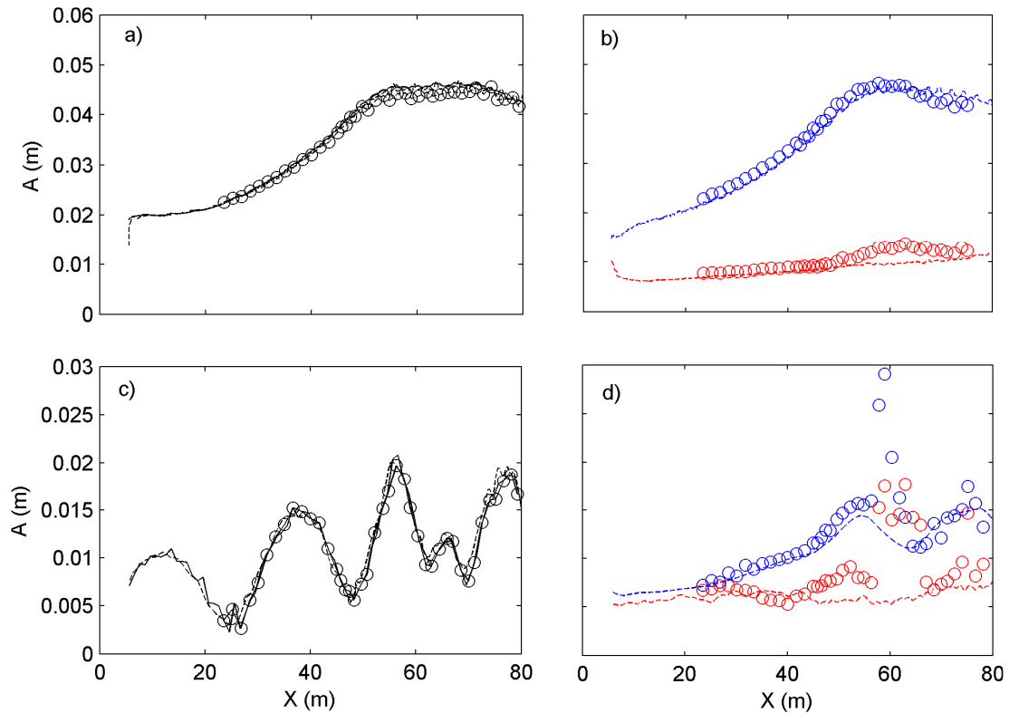
Figure 4. Long-wave amplitude A (m) along X (m). Total long-wave amplitude (solid line), reconstructed from RT (dashed line) and from Guza84 (circles) for a) A2 and c) B2. Incoming and outgoing waves amplitude, for b) A2 and d) B2, estimated from Guza et al. (1984) (circles) and from Radon (dashed line). Red is outgoing component and blue is ongoing.
