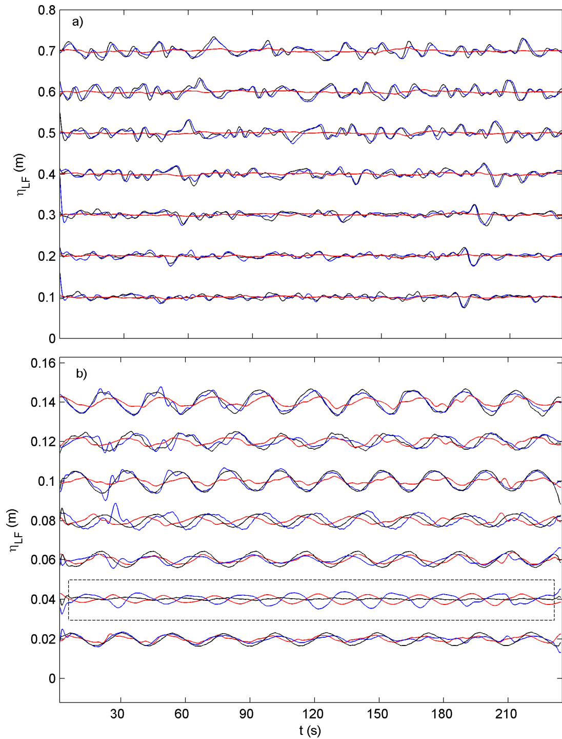
Figure 3. Low frequency ( f < 3/5 f_p ) surface elevation \eta_{LF} (m) timeseries every 10 m from the most offshore sensors to the beach (bottom to top) for the a) random A2 and b) bichromatic B2 cases: (black) total, (blue) incoming and (red) outgoing components. Dashed rectangle indicates the location of standing long wave node.
