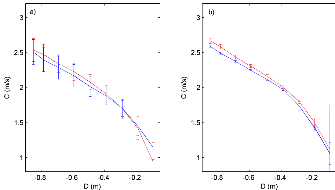
Figure 1. Average celerity derived from wave-by-wave estimation for a) A2 and b) B2. Errorbars stand for dispersion. Red line is RT-derived, blue line trajectory tracked.
