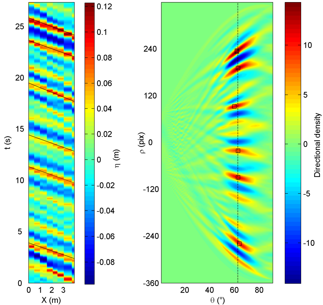
Figure 1. Illustration of the use of Radon Transform for wave-by-wave celerity estimation. a) Spatiotemporal field of short-wave surface elevation and b) its Radon Transform expressed as a directional density (or distribution). In a) crest trajectories (black lines) are shown and corresponding local maxima (black squares) locations give crests propagation angle. In b) the dashed line represents the mean detected crests angle.
