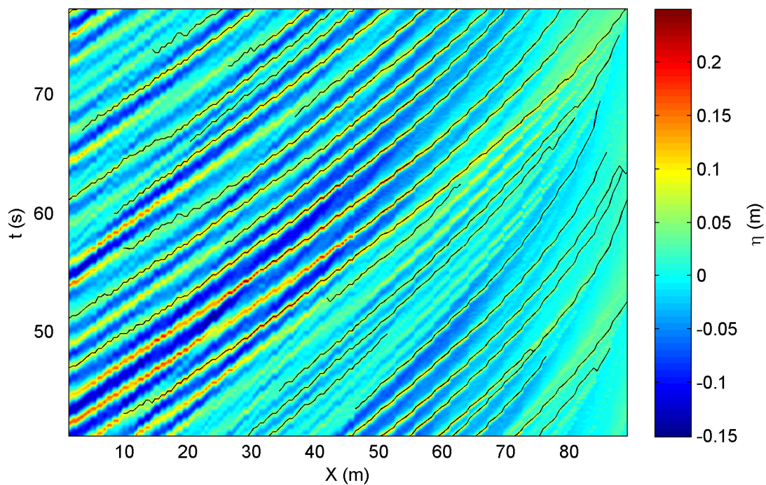
Figure 5. Illustration of the crest tracking method: unfiltered spatiotemporal surface elevation along the cross-shore direction X (m) for the random A2 case. Superimposed black lines stand for the detected crests that passed the quality control.
